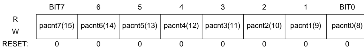
Figure 3-17 Pulse Accumulators Count Register 3 (PACN3)
