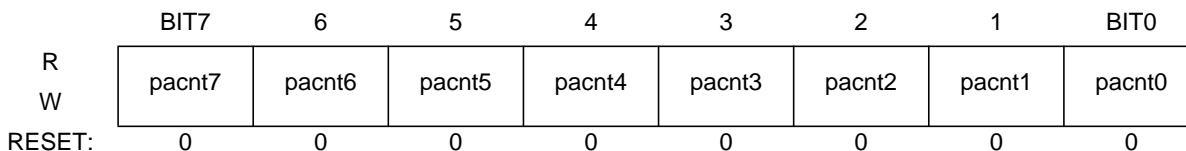
Figure 3-18 Pulse Accumulators Count Register 2 (PACN2)
