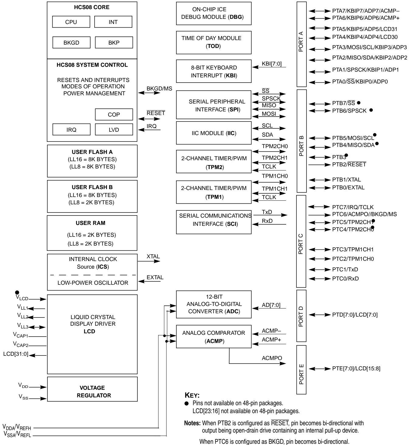
Figure 15-1. MC9S08LL16 Series Block Diagram Highlighting SPI Block and Pins
