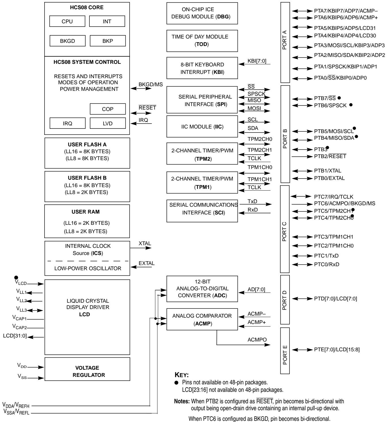
Figure 16-1. MC9S08LL16 Series Block Diagram Highlighting TPMx Blocks and Pins
