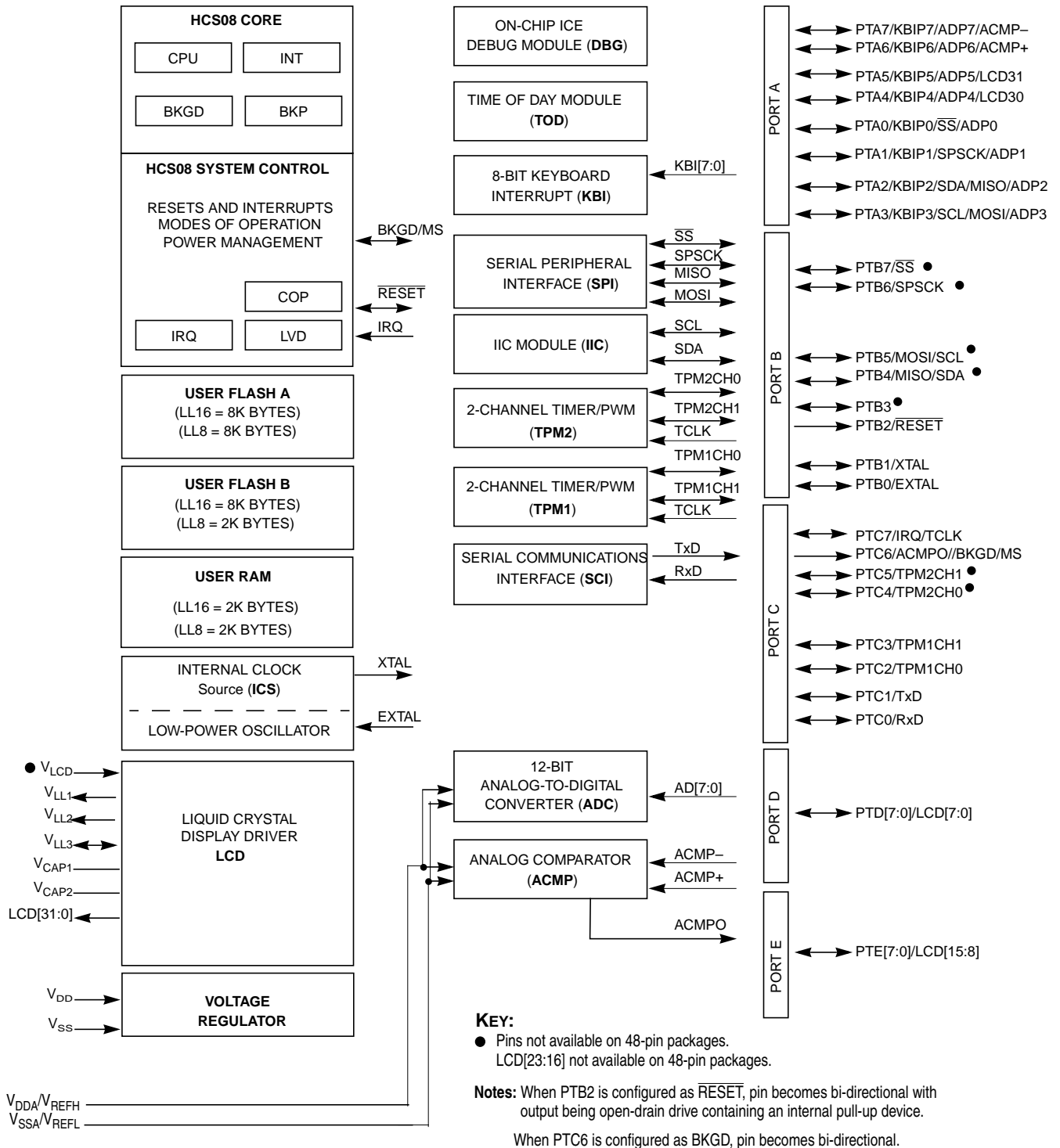
Figure 1-1. MC9S08LL16 Series Block Diagram
