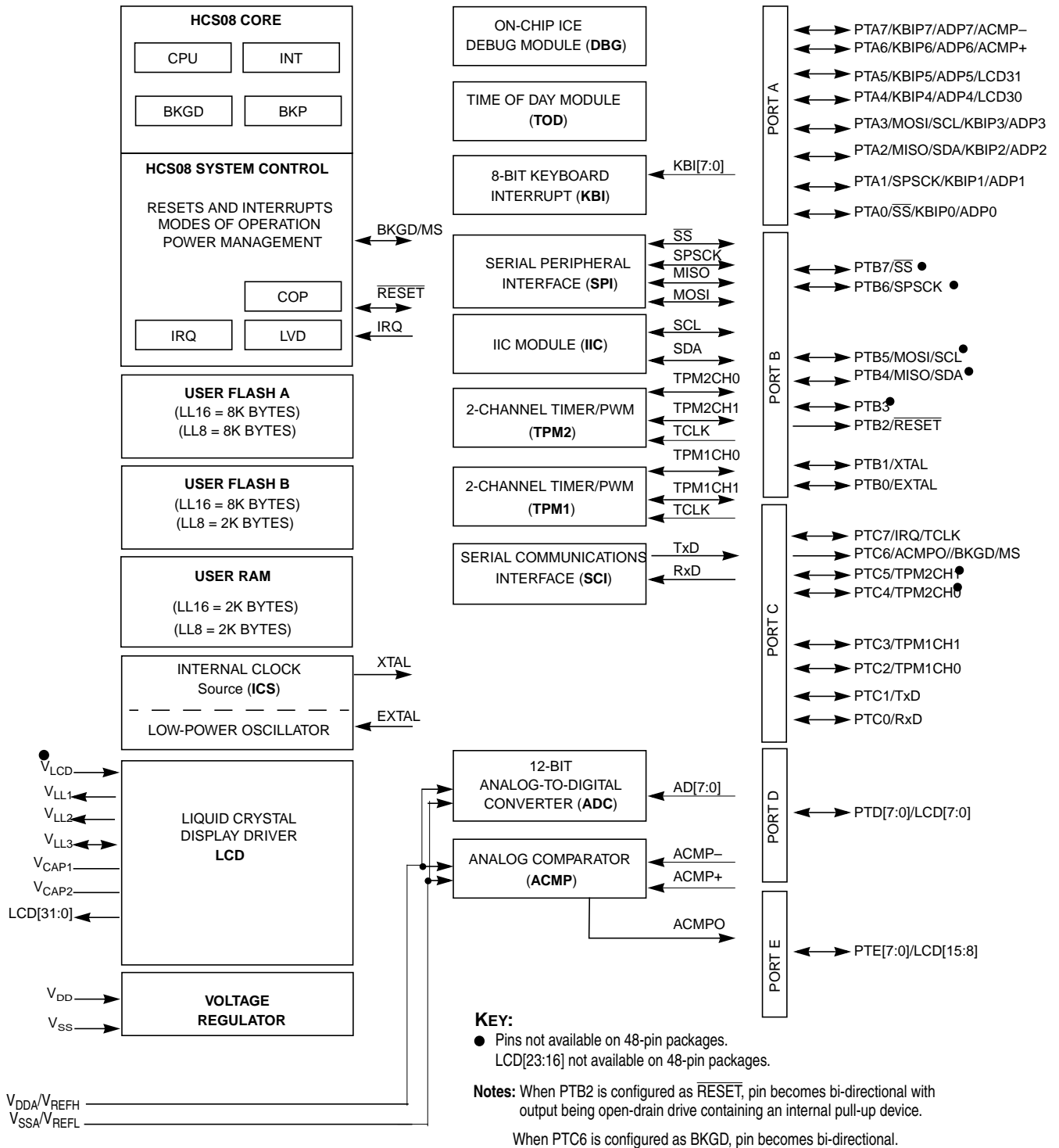
Figure 17-1. MC9S08LL16 Block Diagram Highlighting TOD Block and Pins
