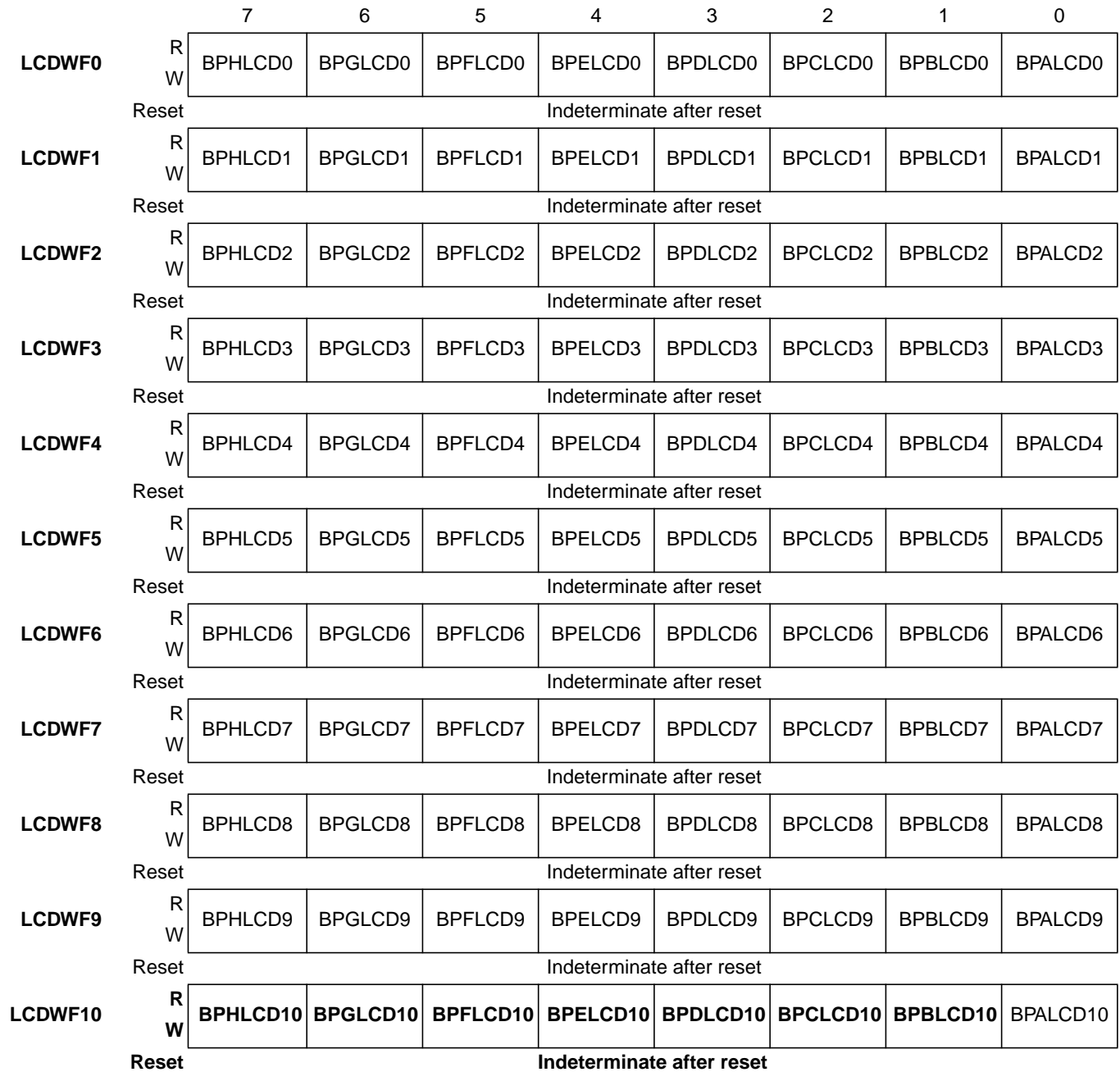
Figure 13-11. LCD Waveform Registers (LCDWF[63:0])
