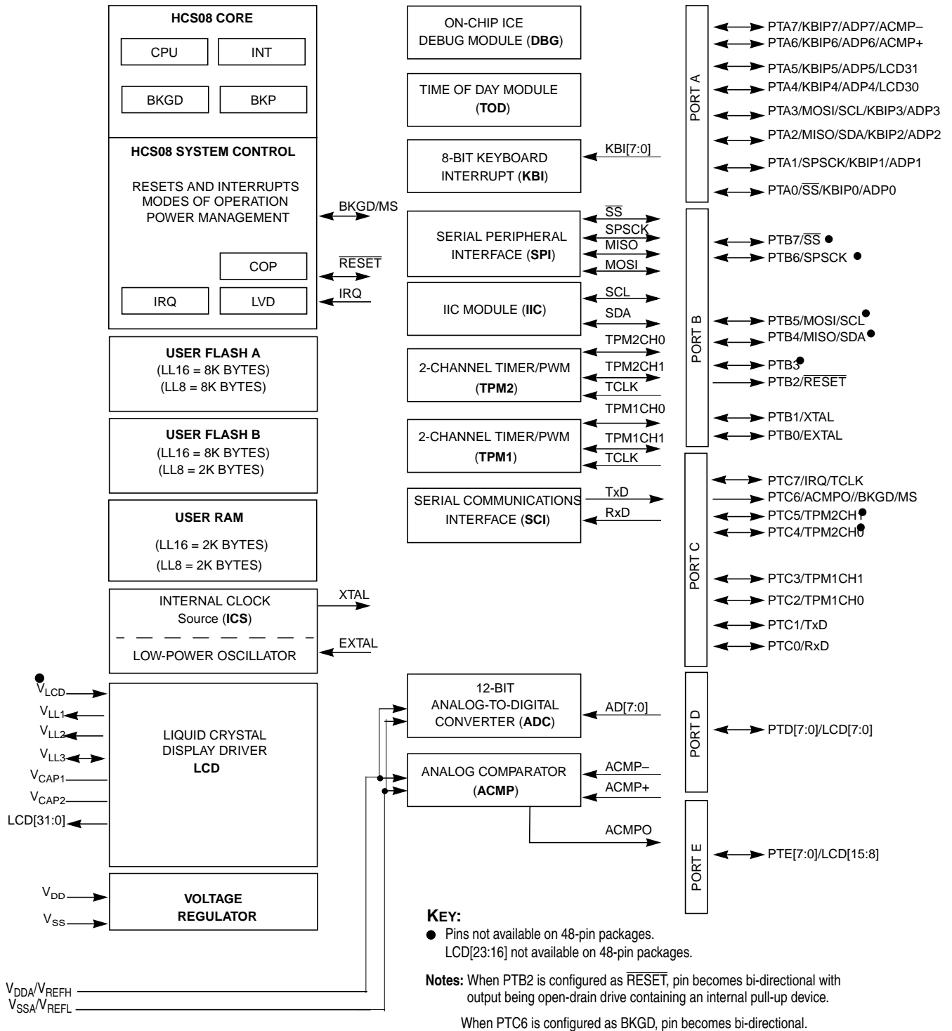
Figure 13-1. MC9S08LL16 Block Diagram Highlighting LCD Block and Pins
