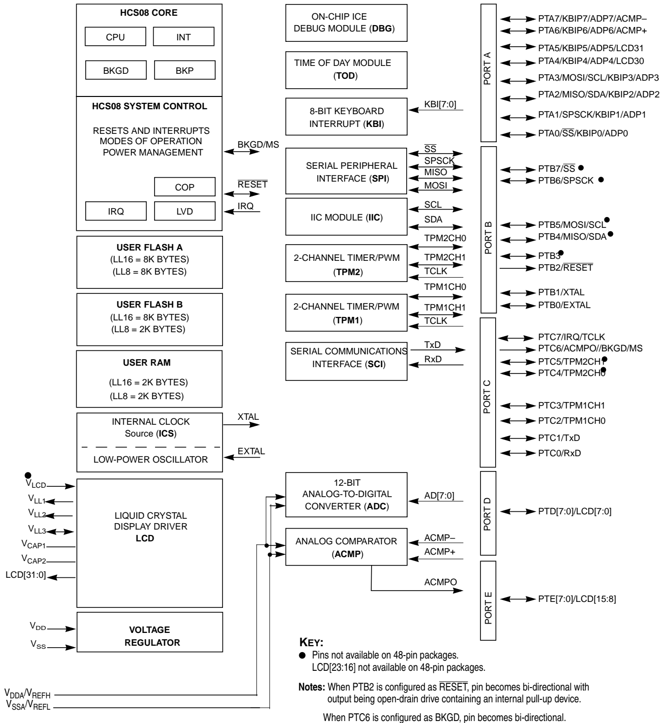
Figure 11-1. MC9S08LL16 Series Block Diagram Highlighting ICS Block and Pins
