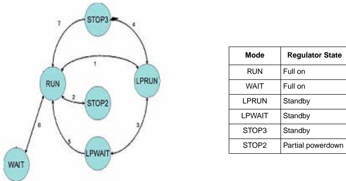
Figure 3-1. Allowable Power Mode Transitions for the MC9S08LL16 Series
